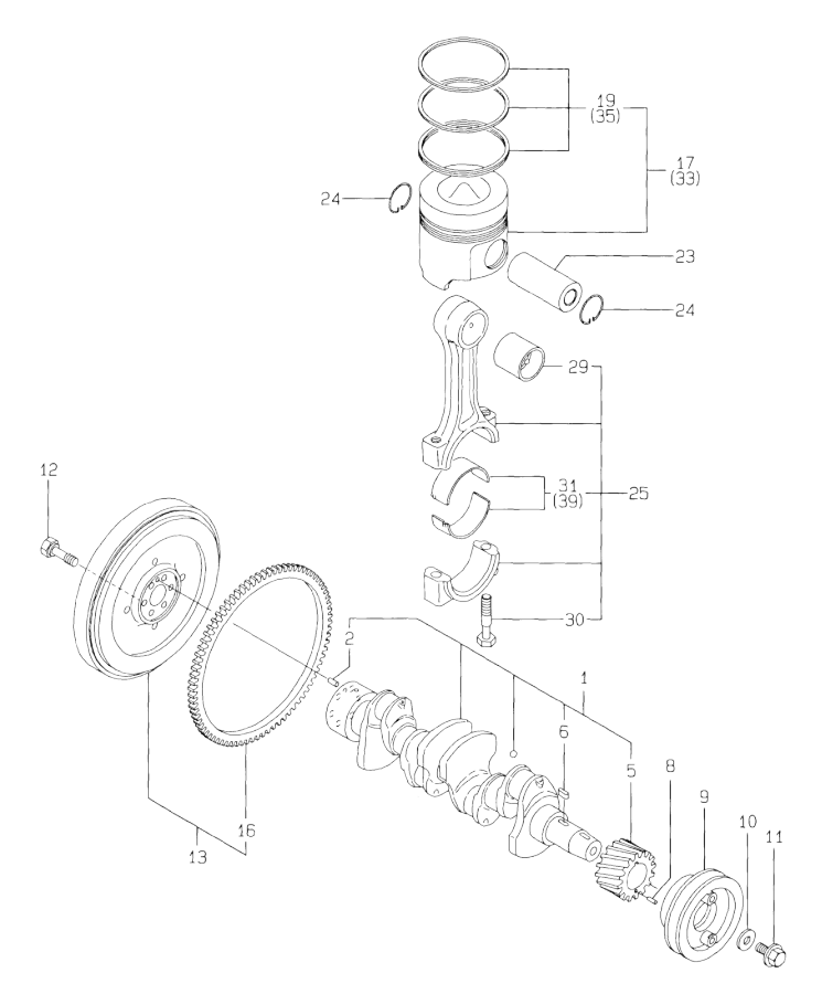
Fig.45. CRANKSHAFT & PISTON
