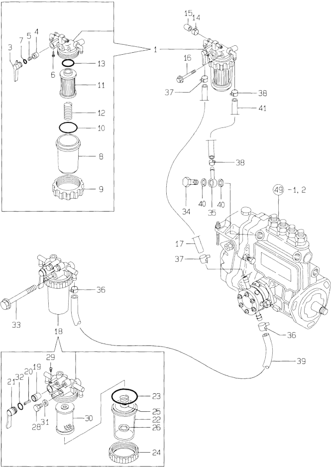
Fig.52. FUEL LINE
