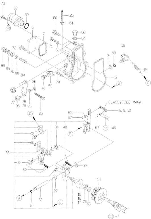
Fig.12. GOVERNOR
