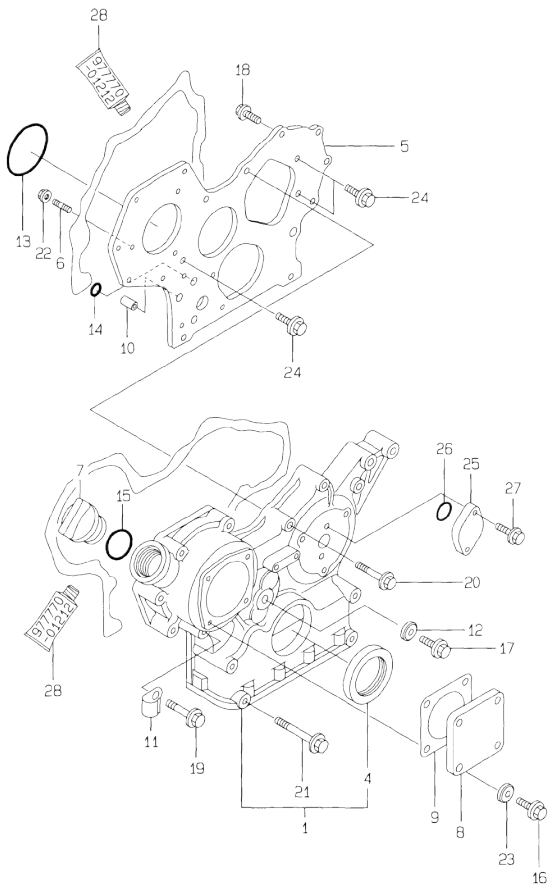
OCB10-M60300 4TNE84T-GB1(S) Fig.38. GEAR HOUSING
