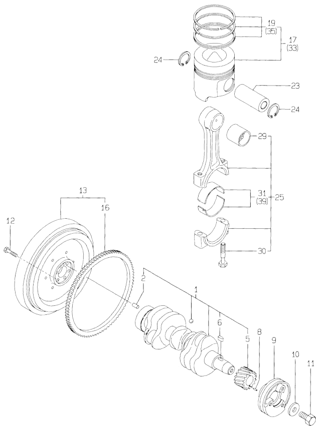
Fig.8. CRANKSHAFT & PISTON
